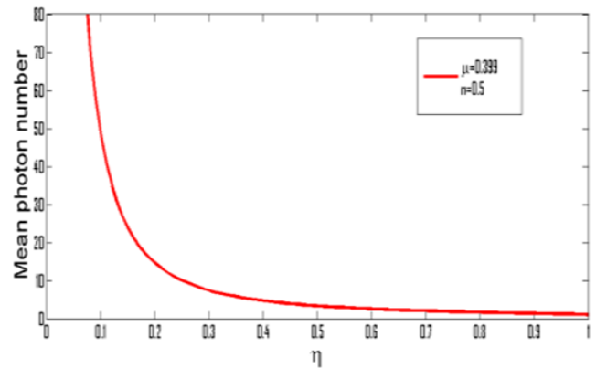
Figure. 4. The mean photon number versus \eta for A = 100 , \kappa = 0:8 , \mu = 0:399 , and \bar{n}_{th} = 0:5
