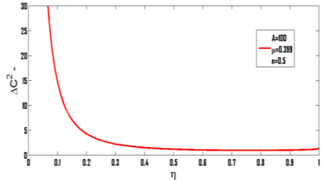
Figure 2. The quadrature variances versus \eta for A = 100 , \kappa = 0.8 , \mu = 0.399 , and \bar{n}_{th} = 0.5
