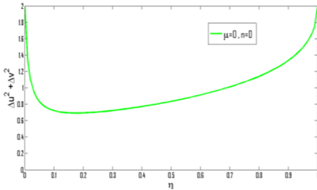
Figure. 9. \Delta u^2 + \Delta v^2 of two-mode light in the cavity at steady state versus \eta for \kappa = 0.8 , A = 100 , \mu = 0 , and n = 0
